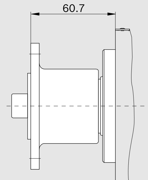
Coupling Flange
